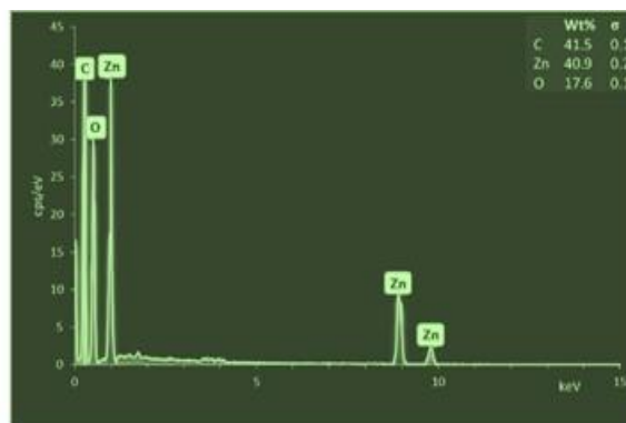
Fig. 5b: EDS of ZnNPs
