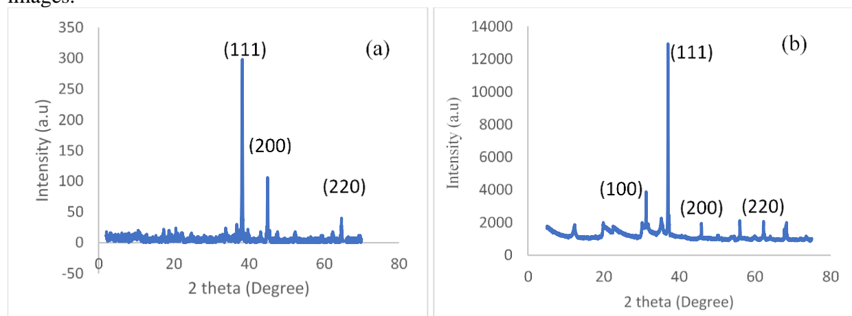
Fig. 4a: XRD pattern of AgNPs
