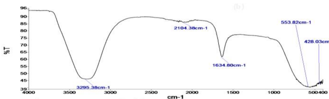
Fig. 2b. FT-IR spectrum of synthesized AgNPs
