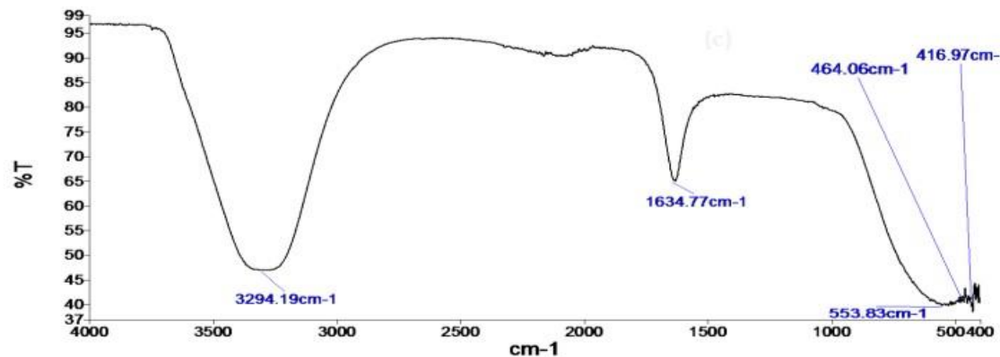
Fig. 2c. FT-IR spectrum of synthesized ZnNPs
