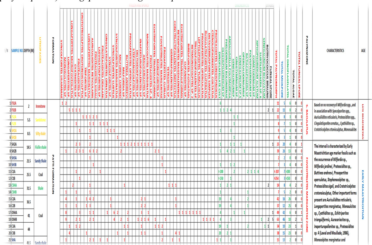
Fig. 3: Palynomorph distribution chart, palynozonation, Age and paleoenvironment of deposition of Patti Formation.
