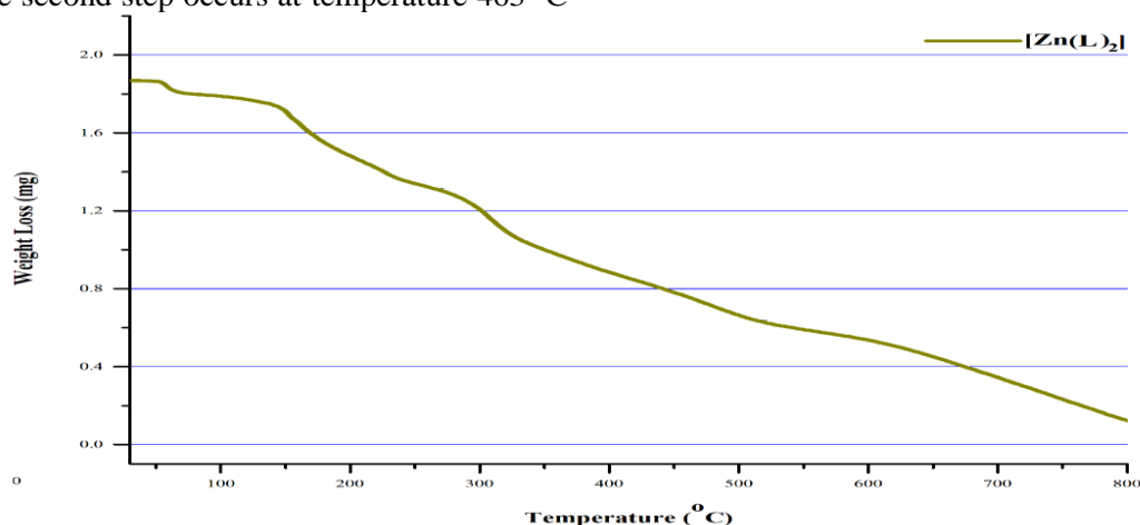
Fig. 4: Thermogravimetric analysis of [Zn(L) 2 ].2H 2 O complex
