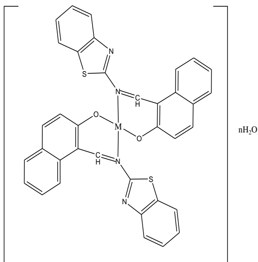
Fig. 6: Proposed structure of [\text{Cu}(\text{L})_2] and [\text{Zn}(\text{L})_2] \cdot 2\text{H}_2\text{O} Complexes ( \text{M} = \text{Cu}^{2+} or \text{Zn}^{2+} and n = number of water of hydration
