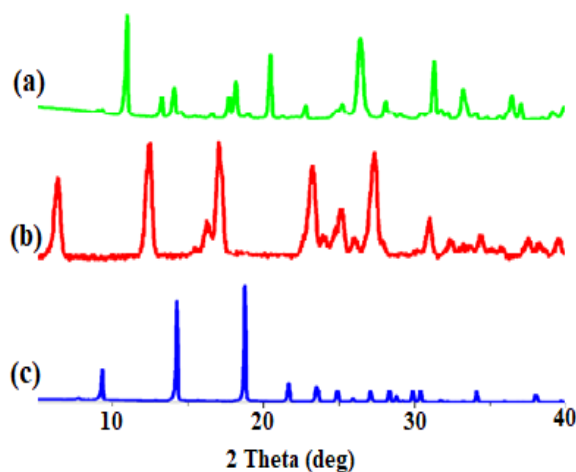
Fig 1. The PXRD Patterns of (a) H_2(L) Schiff base, (b) 2-aminobenzothiazole, (c) 2-hydroxybenzaldehyde showing different PXRD patterns of the Schiff base with respect to the reactants
