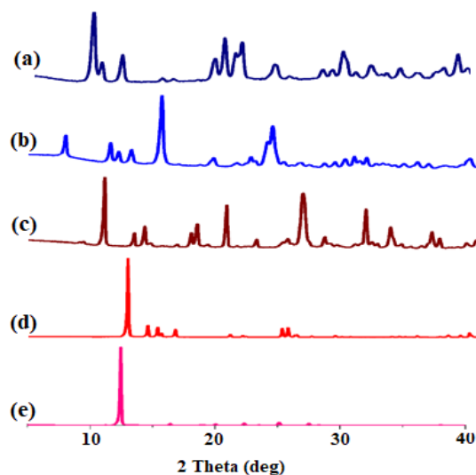
Fig. 2. The PXRD Patterns of (a) [Zn(L)_2] \cdot 2H_2O Complex, (b) [Cu(L)_2] Complex, (c) H_2(L) Schiff base (d) Cu(II) acetate monohydrate, (e) Zn(II) acetate dihydrate showing different PXRD patterns of the synthesized complexes with respect to the derived Schiff base and their respective metal acetate.
