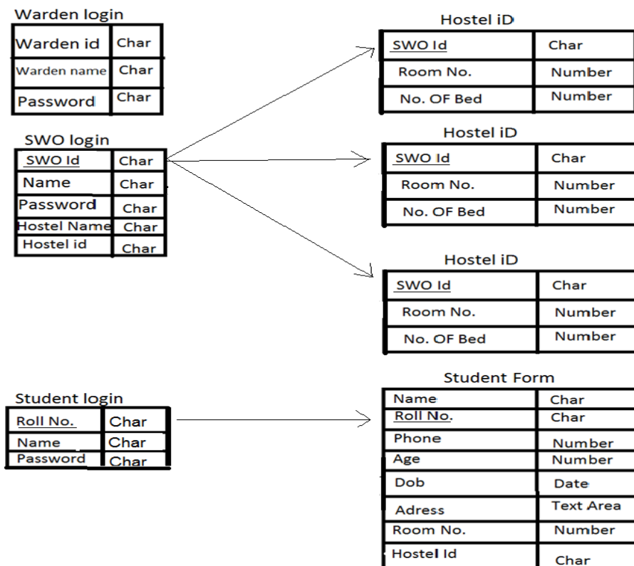
Fig. 1: ERD shows how login entities are linked with student and hostel records.
