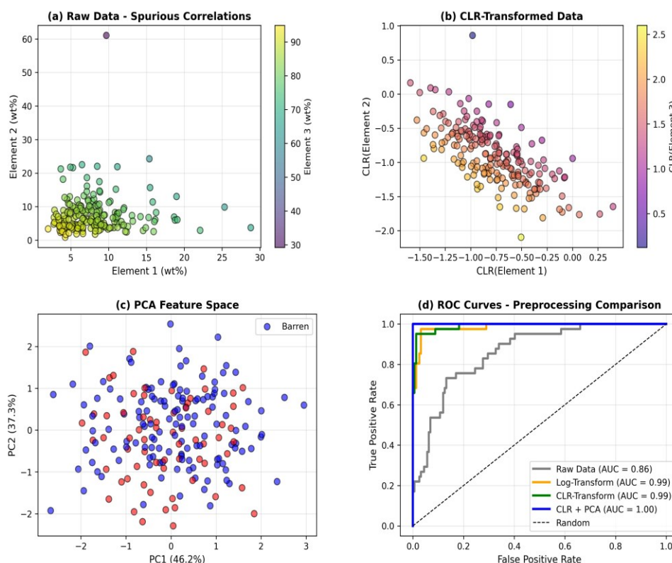
Fig. 3: Comparison of preprocessing techniques on geochemical data. Image (a) Scatter plots of the raw data of closure effects and spurious correlations. (b) CLR-transformed data that shows the elimination of compositional artifacts. (c) Sample in PCA dimensionality reduced feature space with a clustering of samples. (d) Receiver Operating Characteristic (ROC) curves of performance of models with various preprocessing strategies (Based on methodologies from Fizmoser et al. , 2009; Grunsky and de Caritat, 2020).
