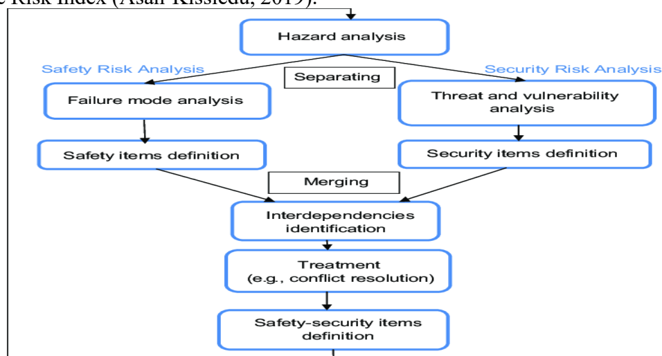
Fig.2: Integrated safety-security risk assessment for industrial control system (Bhosale, Kastner & Sauter, 2023)
