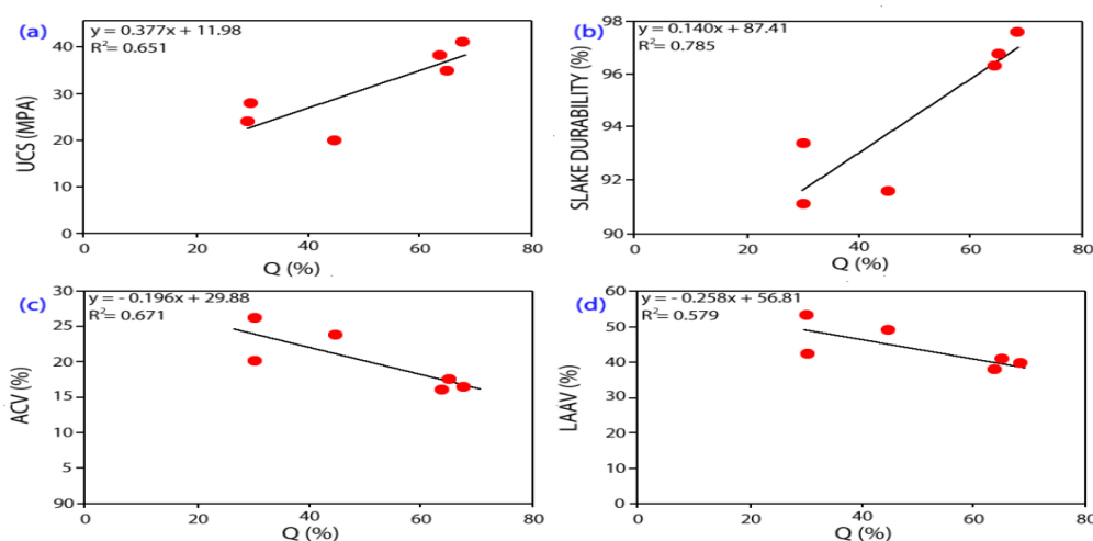
Fig. 6 Relationship between mechanical parameters against quartz (a) UCS vs Quartz; (b) Slake durability vs Quartz; (c) ACV vs Quartz; (d) LAAV vs Quartz
