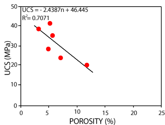
Fig. 12: Relationship between UCS and Porosity
