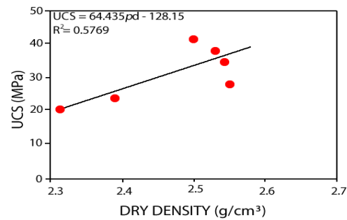
Fig. 9b: Relationship between UCS and dry density
