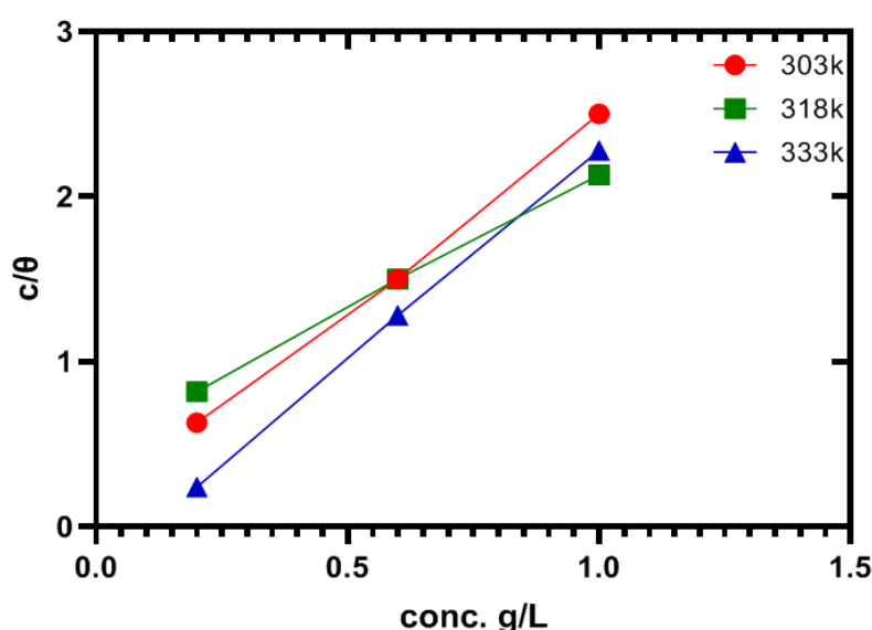
Fig. 5: Langmuir isotherm of in different concentrations of Ficussur in 1 M HCl in 2hrs
