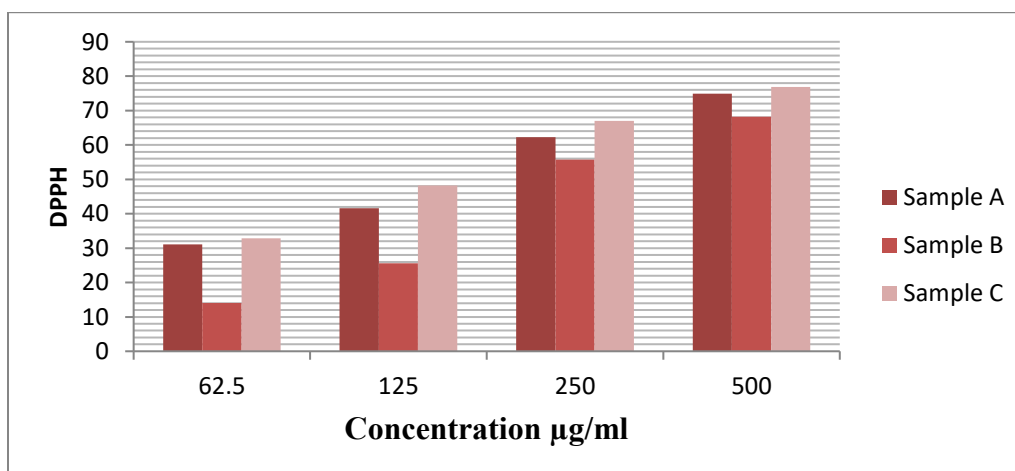
Figure 2:Column chart showing the concentration-dependent DPPH radical scavenging activity of samples A, B and C
