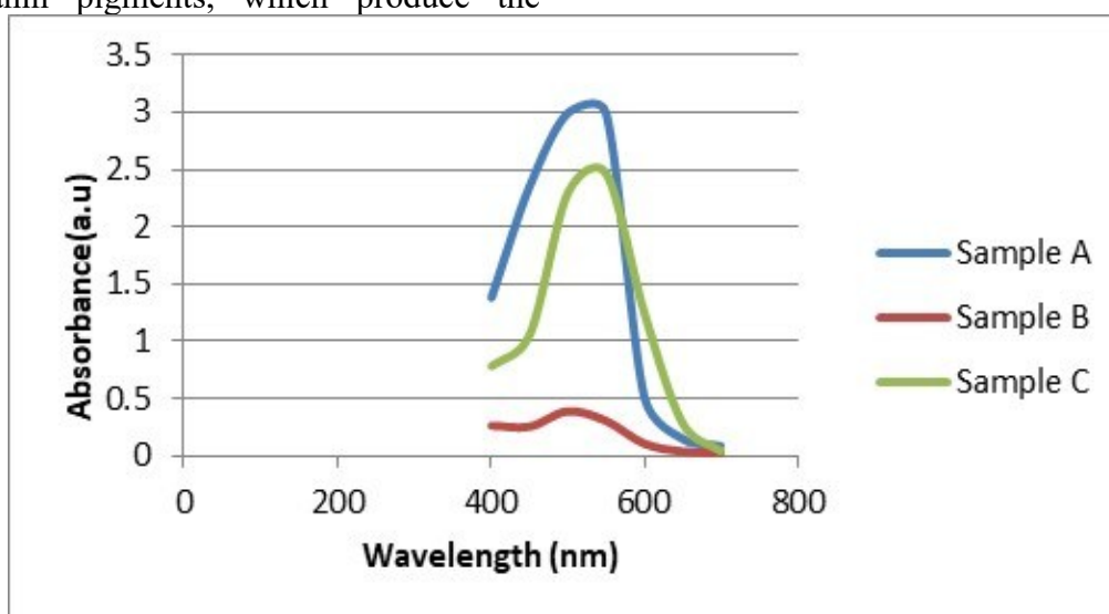
Fig. 1: UV-Visible Absorption spectrum
