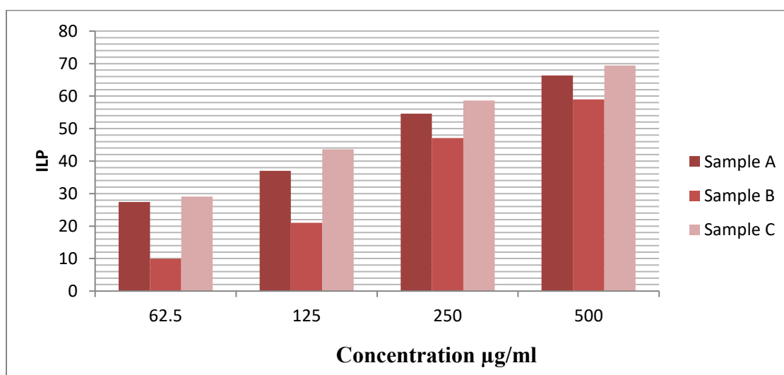
Fig.4: Column chart showing the concentration-dependent inhibition of lipid peroxidation of samples A, B and C.
