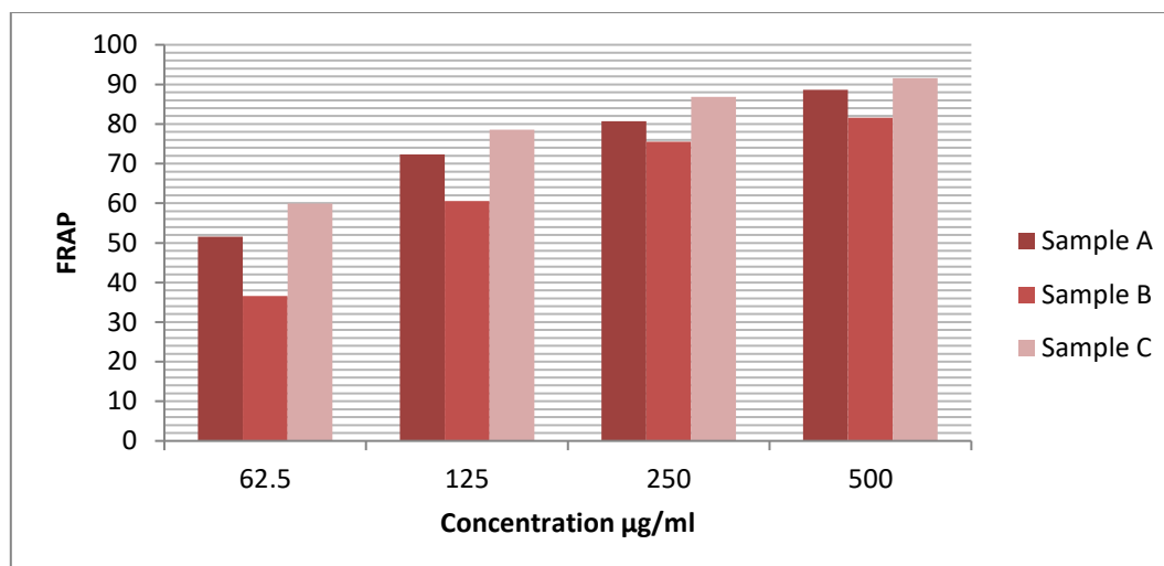
Fig. 3: Column chart showing the concentration-dependent antioxidant power of samples A, B and C
