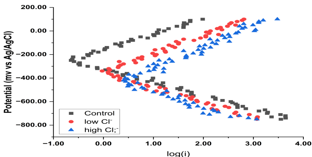
Fig. 4: Potentiodynamic polarization curves of iron embedded in concrete under control, low-chloride, and high-chloride conditions
