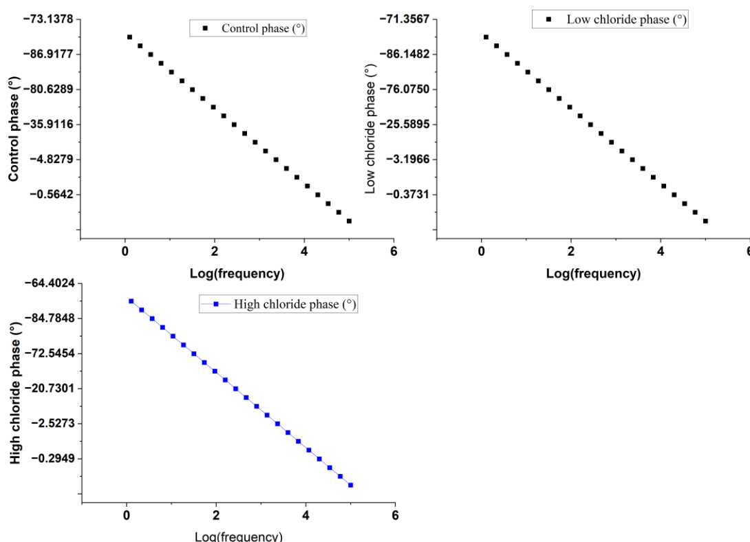
Fig. 3: Bode phase angle as a function of logarithmic frequency for the control, low-chloride, and high-chloride conditions
