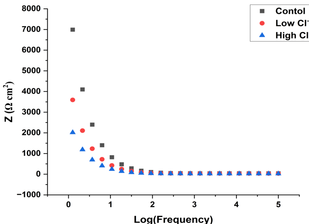
Fig. 2: Bode impedance magnitude as a function of frequency for iron embedded in concrete under control, low-chloride, and high-chloride conditions
