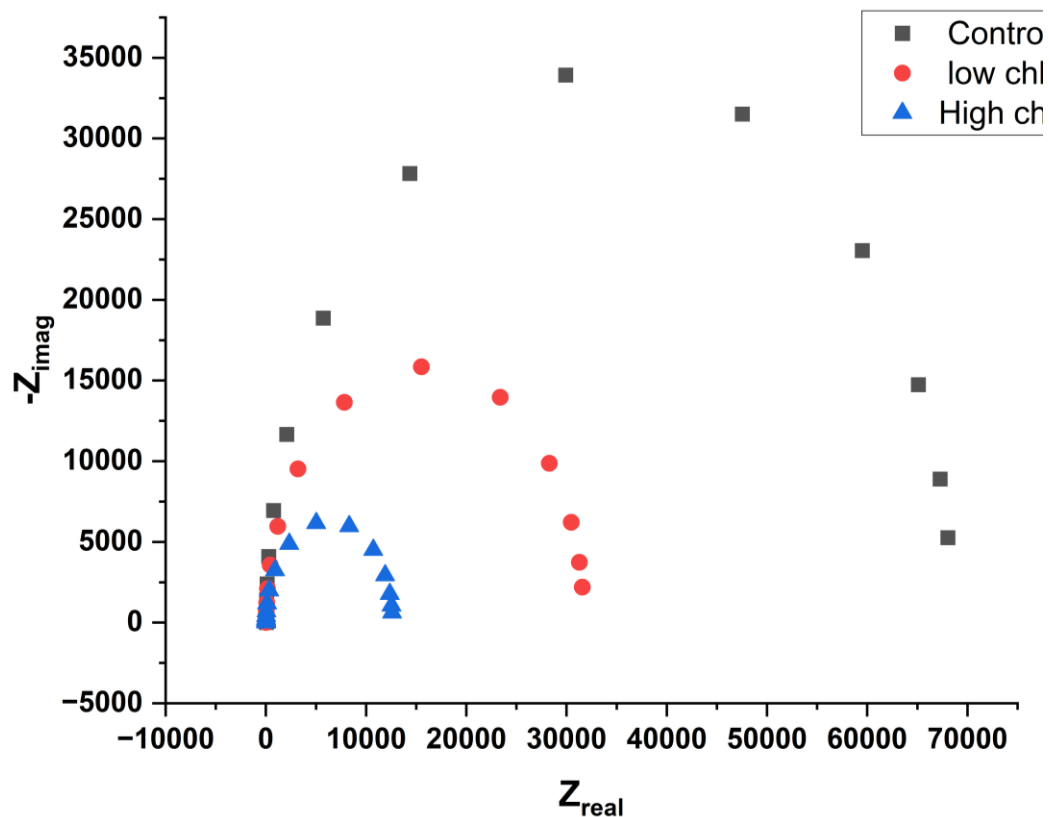
Fig. 1: Nyquist plots of iron embedded in concrete under control, low-chloride, and high-chloride conditions
