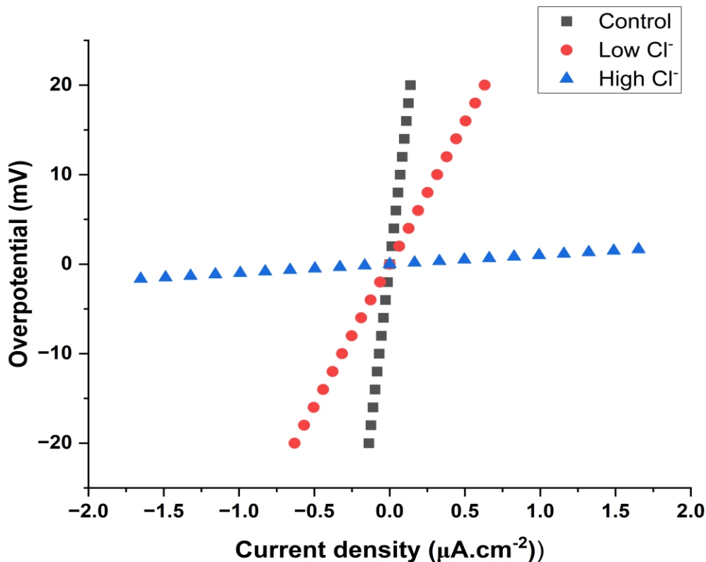
Fig. 5: Current density–overpotential curves of iron embedded in concrete under control, low-chloride, and high-chloride conditions.
