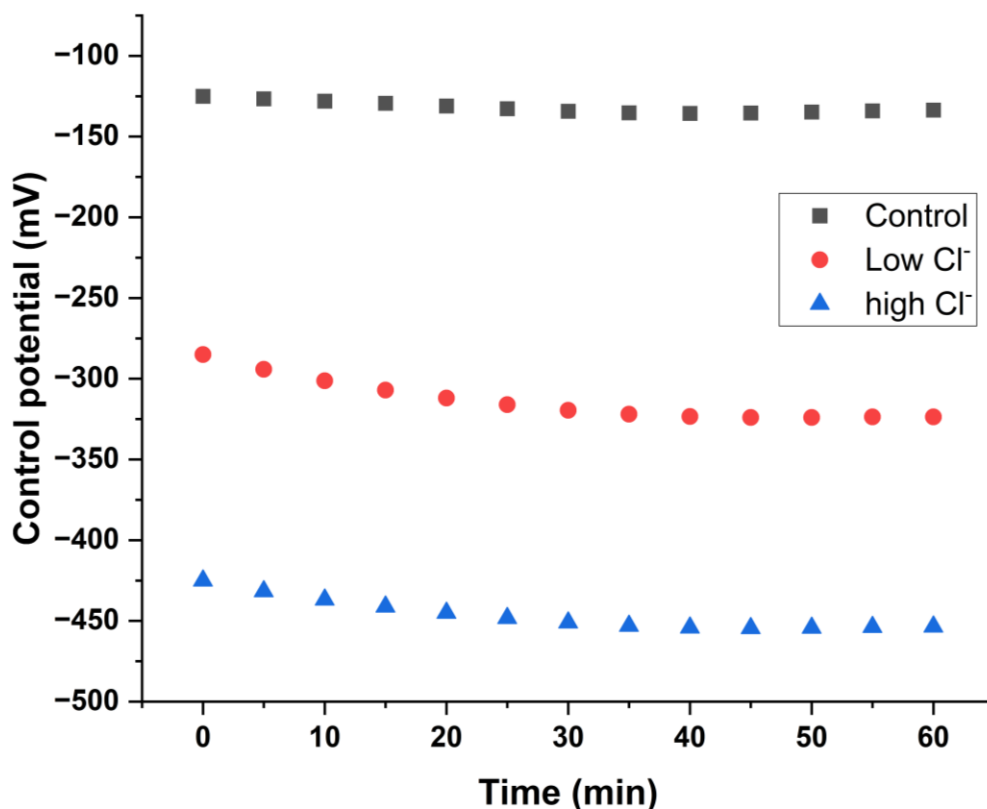
Fig. 6: Variation in open-circuit potential of iron embedded in concrete under control, low-chloride, and high-chloride conditions over 60 minutes.
